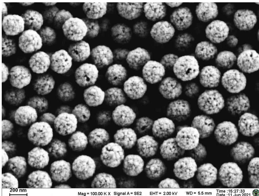
Figure 1. Scanning electron microscope (SEM) image of streptavidin magnetic beads (300 nm).
